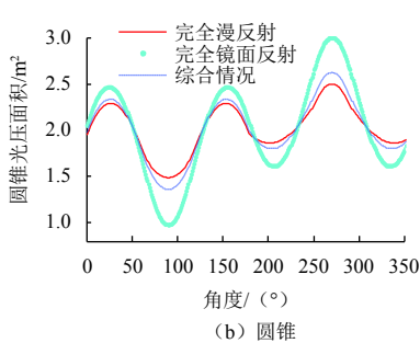
图5 目标光压面积随姿态角 \alpha 变化情况 Fig. 5 Targets' SRP areas changing with attitude angle \alpha
