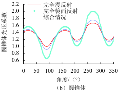
图6 目标光压系数 k 随姿态角 \alpha 变化情况 Fig. 6 Targets' SRP coefficient k changing with attitude angle \alpha
