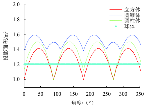
图4 四种目标的投影面积随姿态角变化曲线 Fig. 4 Four targets' projection areas changing with attitude angle \alpha
