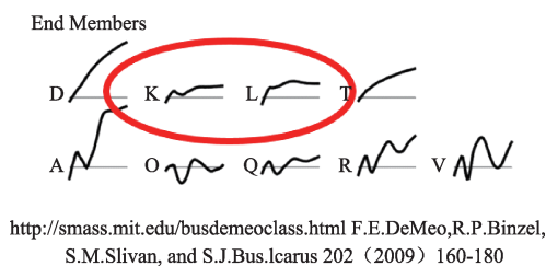
Fig. 8 The K and L types [1]
