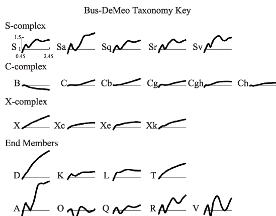
Fig. 1 The Bus-DeMeo asteroid spectral taxonomy [1]
