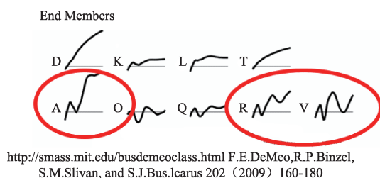
Fig. 7 The A, R, and V types [1]
