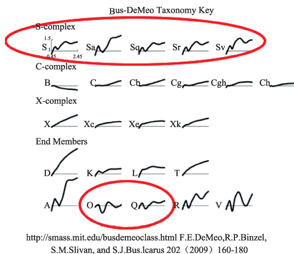
Fig. 6 The S complex and related asteroids [1]
