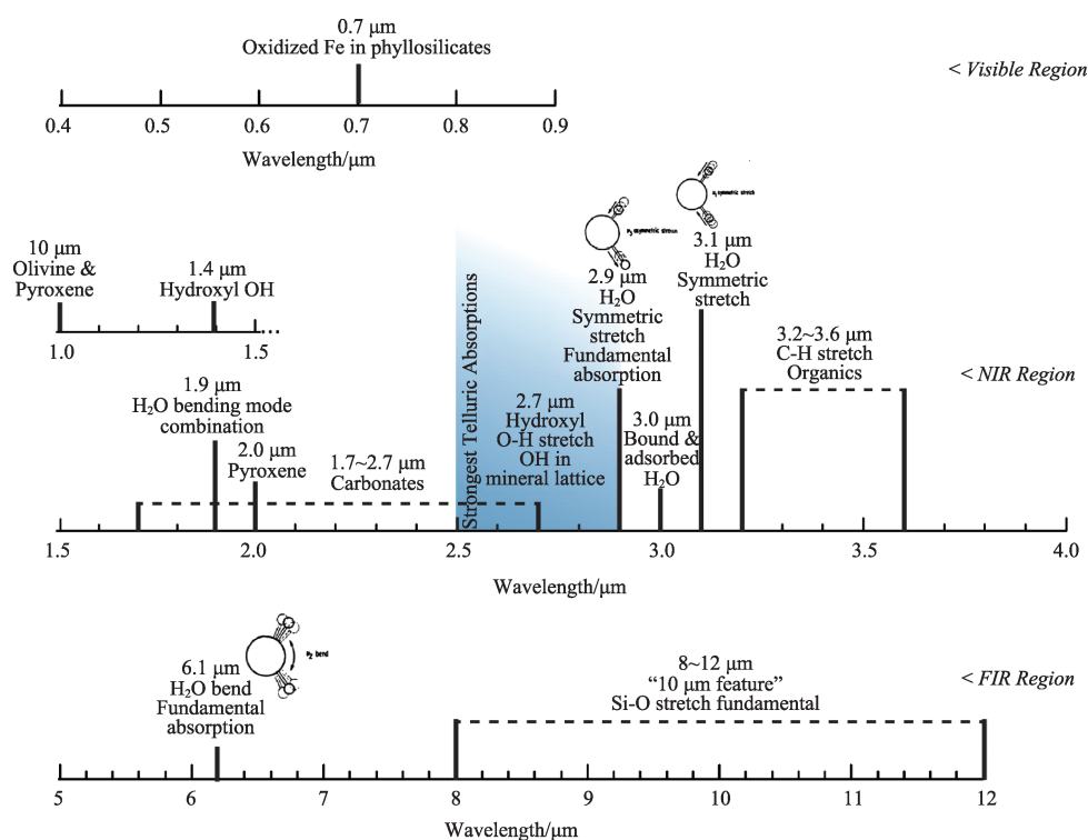
Fig. 3 Spectral absorption features of major asteroidal minerals
