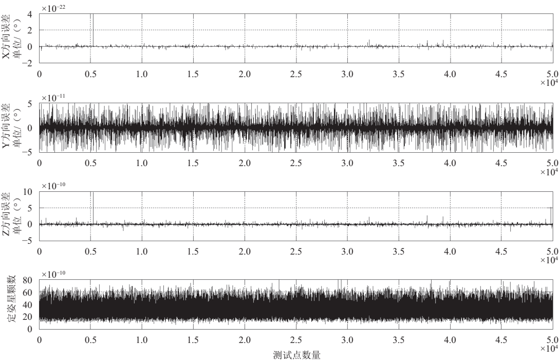
图9 理想姿态与实际姿态的误差 Fig. 9 Error between ideal attitude and actual attitude
