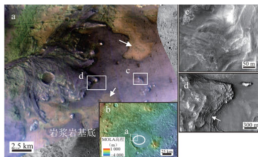
Fig. 1 Locations of landing site candidates discussed in this study
