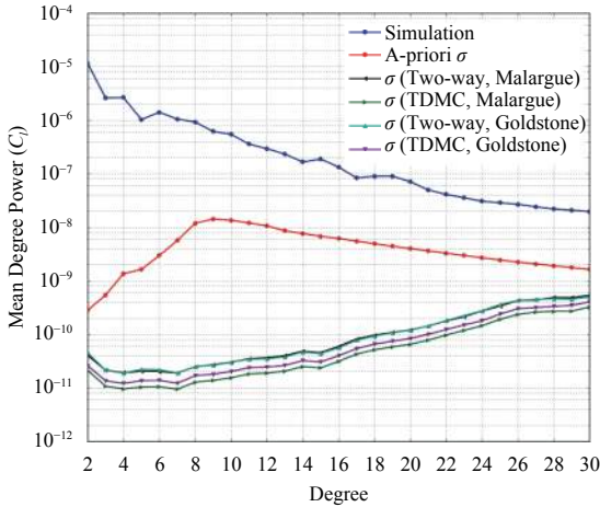
Fig. 2 RMS power of gravity of the simulated HgM005 gravity field (blue), its a priori uncertainty (red), and the associated formal uncertainties obtained through the OD process for the reference two-way link from DSS-25 (Goldstone, cyan) and DSA-3 (Malargüe, black). Green and magenta curves refer respectively to the DSA-3/APEX and DSS-25/APEX TDMC combinations.
