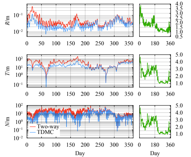
Fig. 3 Left: formal uncertainties for MPO position in Mercury-centered RTN frame considering two-way link from DSS-25 (orange) and DSS-25/APEX TDMC configuration (cyan). Right: gain factor. HGA mechanical noise is calibrated to 25%. For both figures: the radial component is reported at the top, the transversal component in the middle, and the normal component at the bottom.
