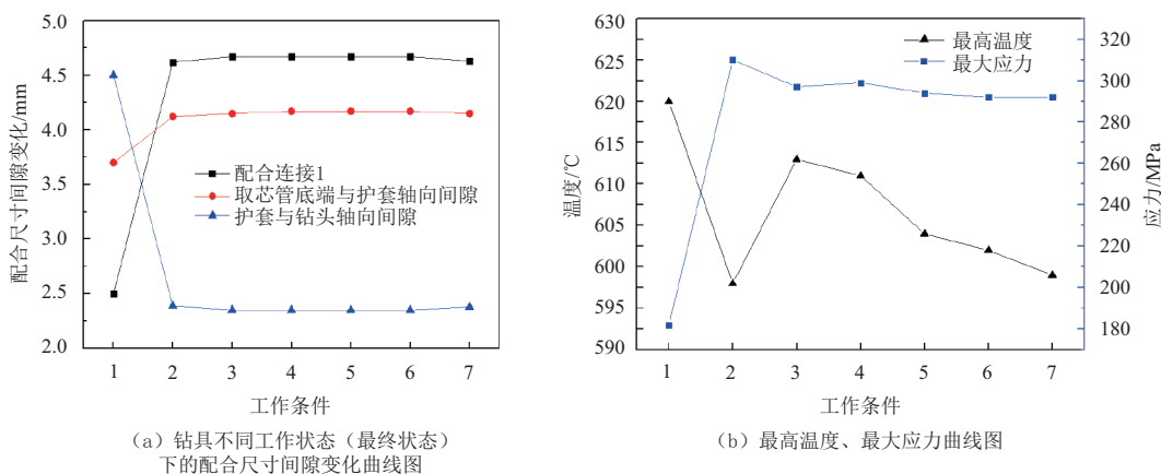
Fig. 6 The displacement, temperature and stress distribution of drilling tool at different stages
